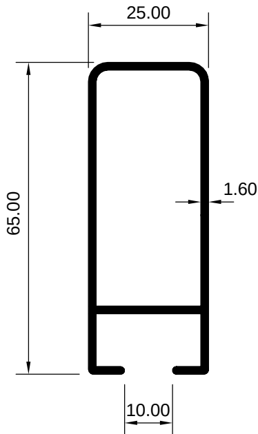
ART 1007953 (KG/MTR = 0.786)
