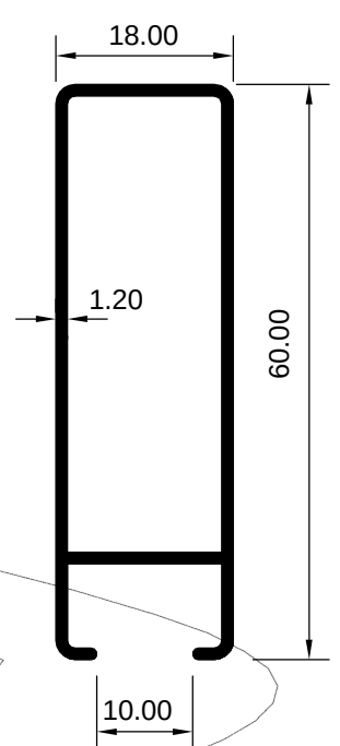
ART 1007955 (KG/MTR = 0.499)
