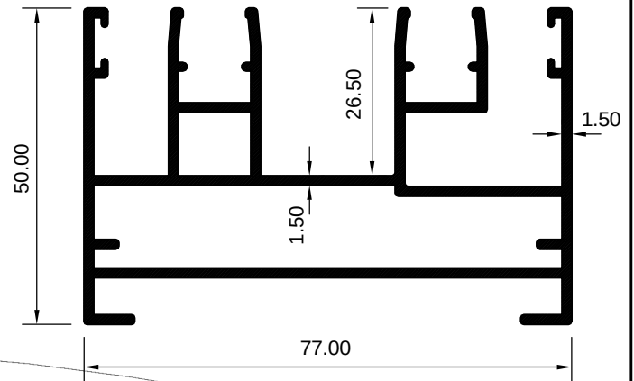
ART 2029338 (KG/MTR = 1.650)
