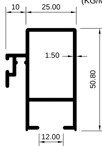
ART 3029044 (KG/MTR = 0.755)
