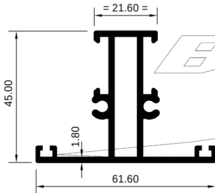
ART 1029334 (KG/MTR = 1.044)
