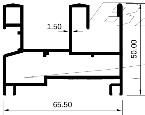
ART 2029412 (KG/MTR = 0.897)
