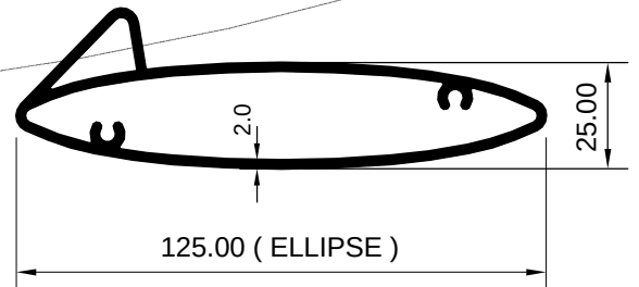
ART 2008029 (KG/MTR = 1.772)
