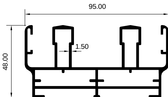
ART 2007997 (KG/MTR = 1.976)
