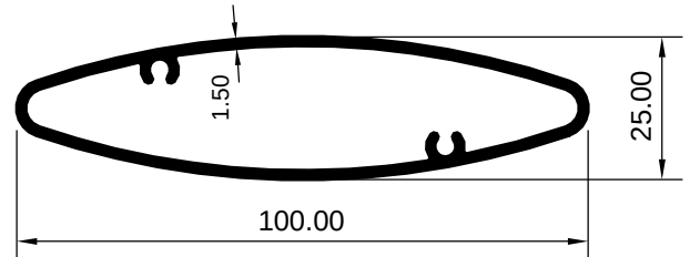
ART 1007989 (KG/MTR = 0.921)
