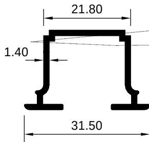
ART 1007886 (KG/MTR = 0.291)
