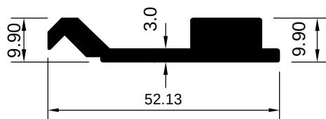
ART 2007917 (KG/MTR = 0.796)
