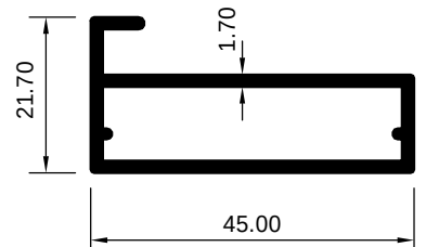
HAD 2007414 (KG/MTR = 0.835)
