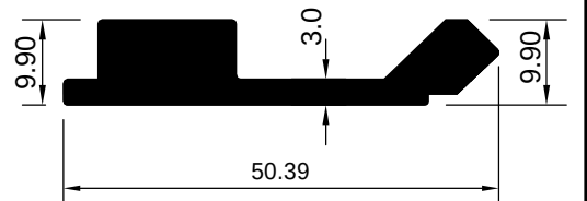
ART 2007918 (KG/MTR = 0.810)
