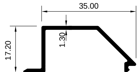
ART 1007910 (KG/MTR = 0.238)
