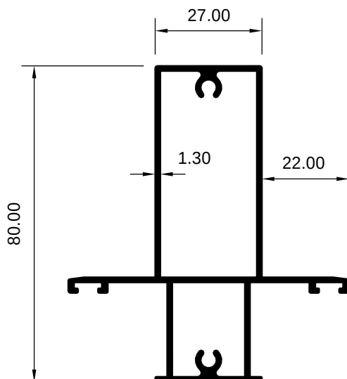
ART 1029222 (KG/MTR = 1.136)
