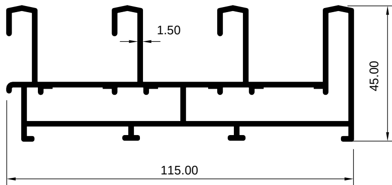
ART 2008001 (KG/MTR = 1.960)
