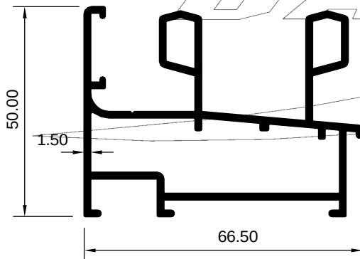
ART 2007987 (KG/MTR = 1.336)
