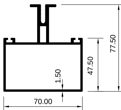
ART 2029141 (KG/MTR = 1.547)
