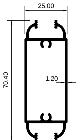
ART 2008052 (KG/MTR = 0.747)
