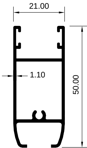
ART 1007867 (KG/MTR = 0.487)
