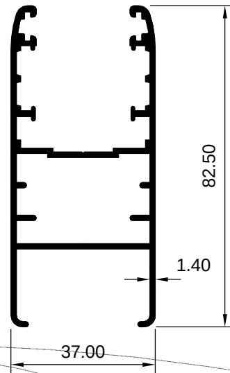
ART 2007965 (KG/MTR = 1.160)
