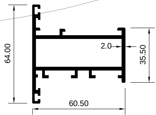
ART 2008042 (KG/MTR = 1.401)
