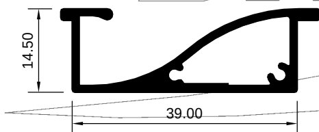
HAD 2007583 (KG/MTR = 0.806)
