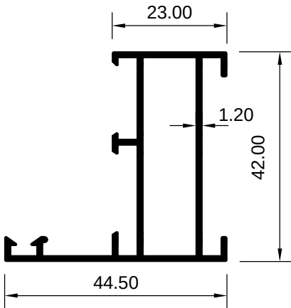
ART 1007956 (KG/MTR = 0.574)
