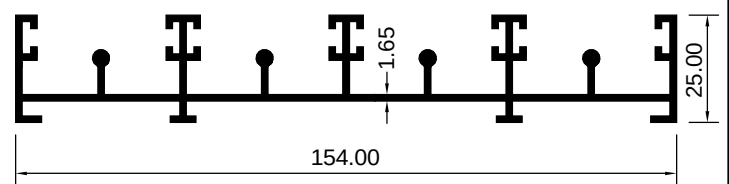
ART 2007767 (KG/MTR = 1.885)
