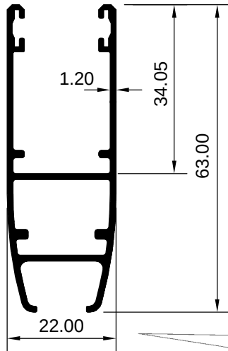
ART 1007913 (KG/MTR = 0.628)
