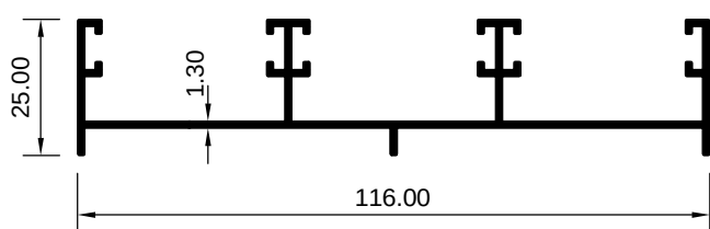
ART 2007796 (KG/MTR = 1.043)
