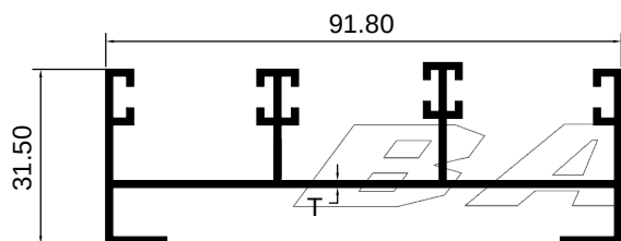
3 TRACK TOP
