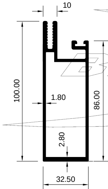
ART 2029111 (KG/MTR = 1.624)
