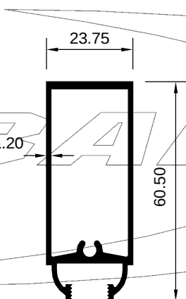
ART 1007786 (KG/MTR = 0.690)
