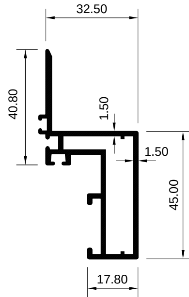
ART 1029347 (KG/MTR = 0.872)
