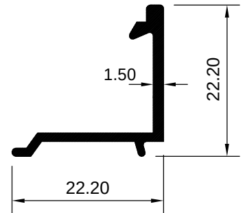
ART 1007850 (KG/MTR = 0.180)
