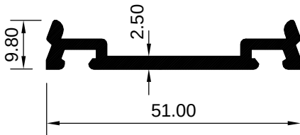
ART 1029143 (KG/MTR = 0.215)
