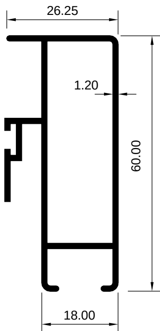
ART 1007954 (KG/MTR = 0.633)
