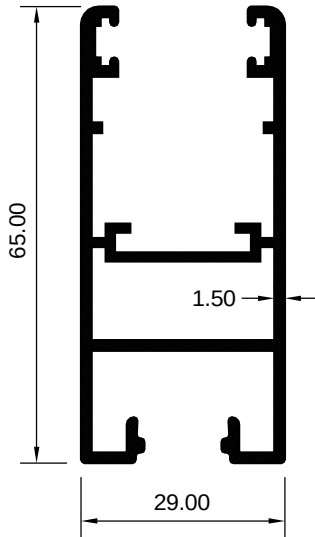
ART 1029315 (KG/MTR = 0.974)
