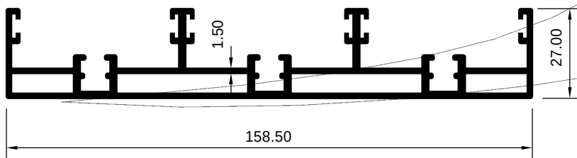
ART 2029291 (KG/MTR = 2.158)
