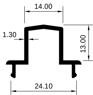
ART 1029226 (KG/MTR = 0.207)
