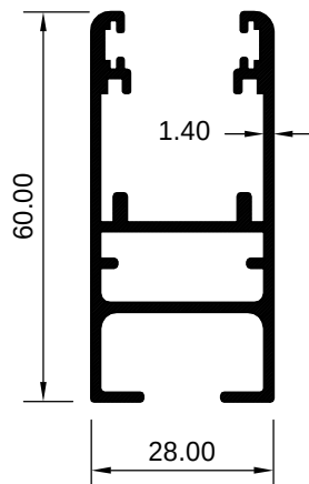
ART 2029412 (KG/MTR = 0.897)
