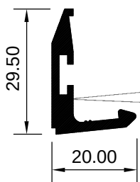
ART 2007939 (KG/MTR = 0.376)
