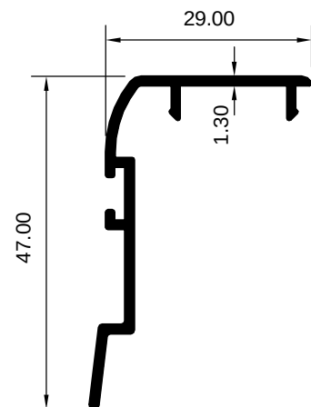
ART 1029036 (KG/MTR = 0.322)
