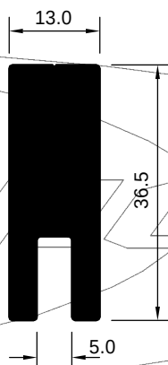
HAD 2007534 (KG/MTR = 1.118)
