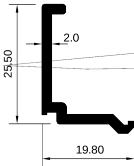
ART 1008016 (KG/MTR = 0.252)
