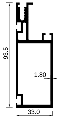
ART 2007715 (KG/MTR = 1.540)
