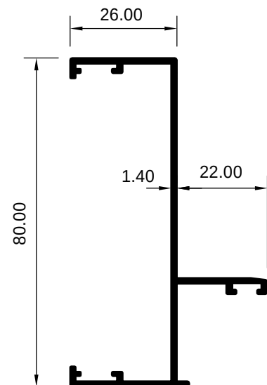
ART 1029219 (KG/MTR = 0.663)
