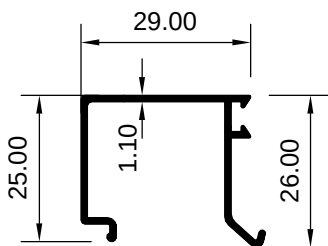
ART 2029385 (KG/MTR = 0.272)
