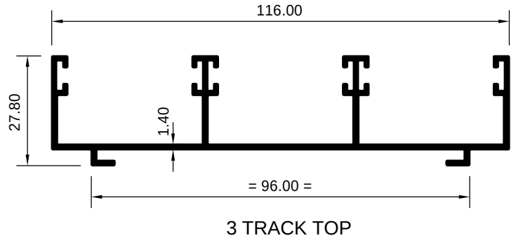
ART 1029042 (KG/MTR = 0.989)
