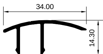
ART 1007780 (KG/MTR = 0.198)
