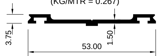
ART 1007862 (KG/MTR = 0.267)
