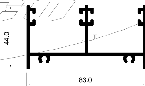
2 TRACK TOP
