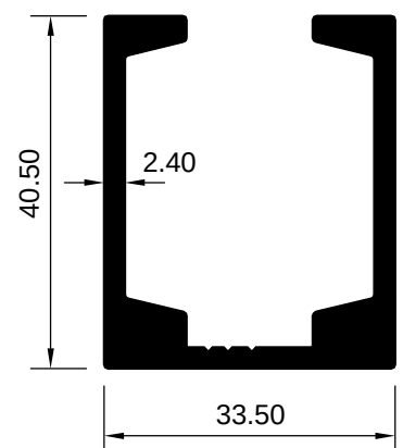
ART 2007993 (KG/MTR = 1.037)
