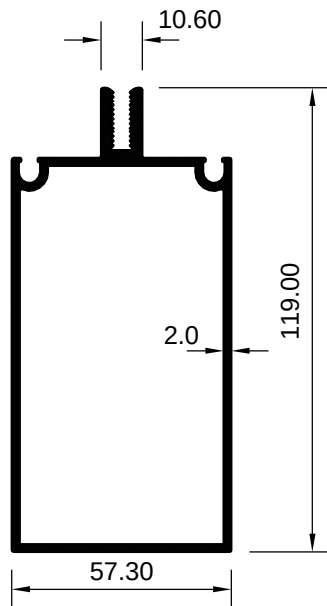
ART 2029259 (KG/MTR = 2.017)
