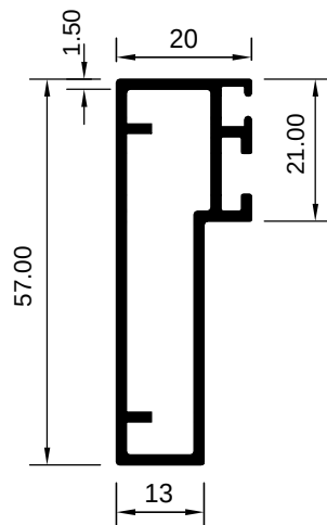
ART 1007895 (KG/MTR = 0.667)
