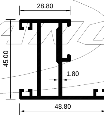
ART 1029335 (KG/MTR = 0.978)
