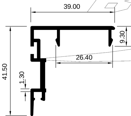
ART 1007996 (KG/MTR = 0.448)
