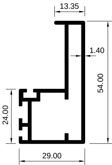
ART 1029142 (KG/MTR = 0.712)
