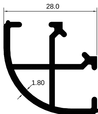
ART 2005211 (KG/MTR = 0.560)
