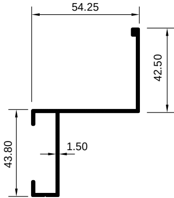
ART 1029331 (KG/MTR = 0.684)
