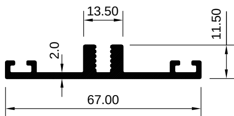
ART 2029341 (KG/MTR = 0.659)
