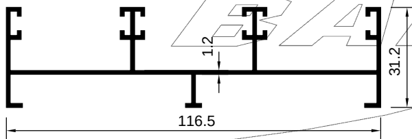
ART 2007701 (KG/MTR = 0.957)
