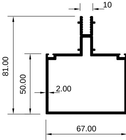
ART 2007938 (KG/MTR = 1.632)
