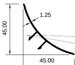
ART 1007775 (KG/MTR = 0.284)
