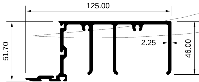
ART 3008031 (KG/MTR = 2.119)
