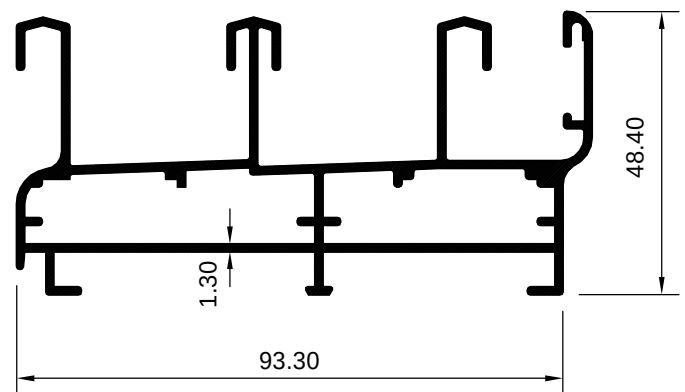
ART 2029411 (KG/MTR = 1.606)
