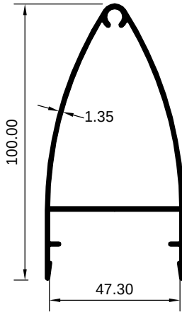
ART 1008074 (KG/MTR = 1.044)
