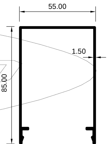
ART 2029140 (KG/MTR = 2.574)
