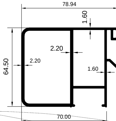
ART 2008009 (KG/MTR = 1.856)
