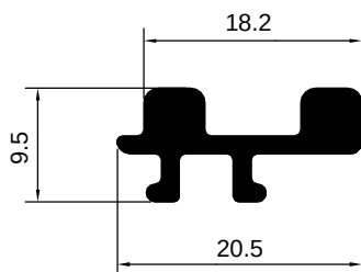
ART 1005209 (KG/MTR = 0.240)
