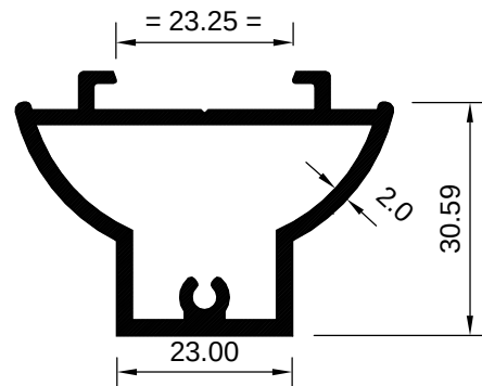
ART 1029158 (KG/MTR = 0.835)
