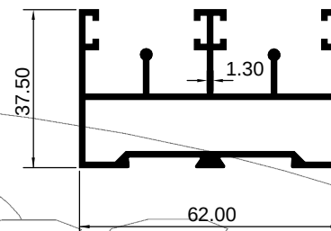
2 TRACK HOLLOW BOTTOM
