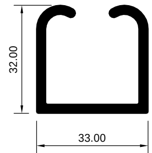
ART 2029048 (KG/MTR = 0.306)
