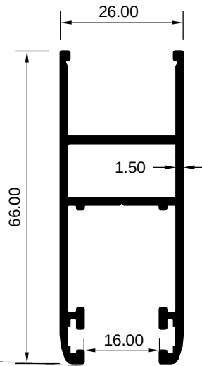
ART 1007983 (KG/MTR = 0.816)
