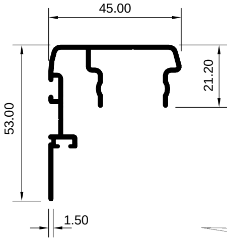
ART 1007964 (KG/MTR = 0.649)
