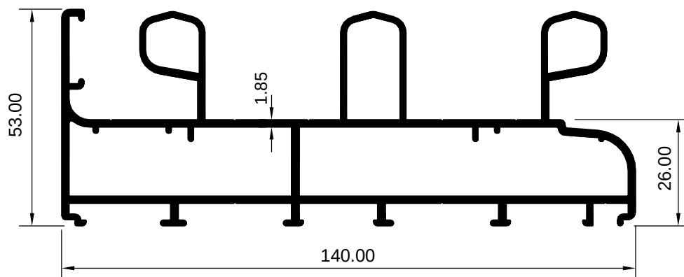
ART 3007968 (KG/MTR = 2.900)
