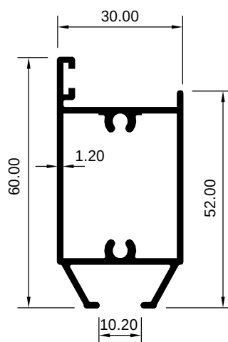
ART 1008090 (KG/MTR = 0.680)
