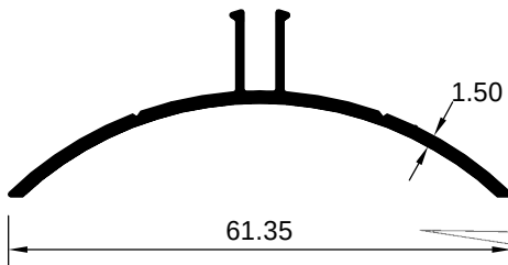
ART 1007848 (KG/MTR = 0.360)
