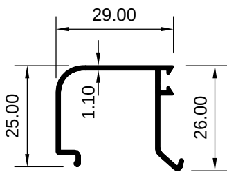
ART 1007893 (KG/MTR = 0.267)
