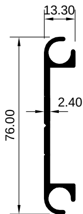
ART 1029168 (KG/MTR = 1.049)
