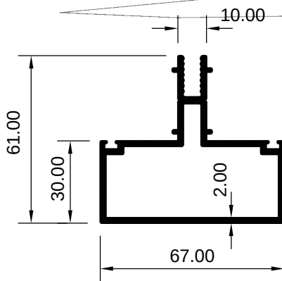
ART 2029341 (KG/MTR = 0.659)
