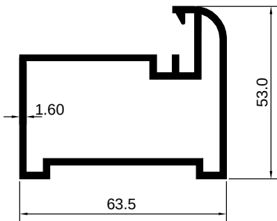
ART 2007731 (KG/MTR = 1.360)
