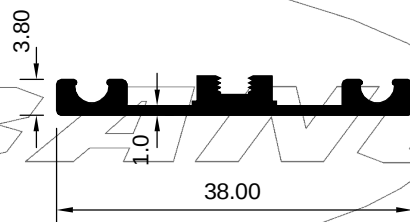
ART 2007763 (KG/MTR = 0.226)
