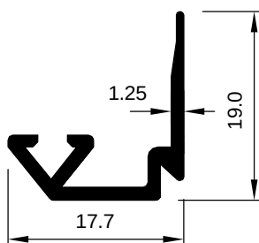
ART 1005505 (KG/MTR = 0.160)
