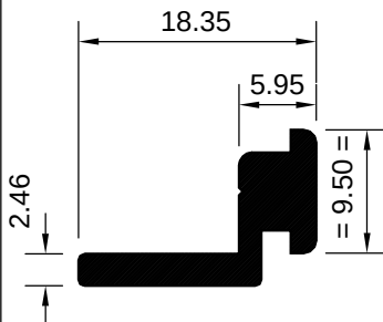
ART 1029105 (KG/MTR = 0.215)
