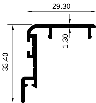
ART 2029410 (KG/MTR = 0.307)
