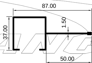
ART 1007722 (KG/MTR = 0.294)
