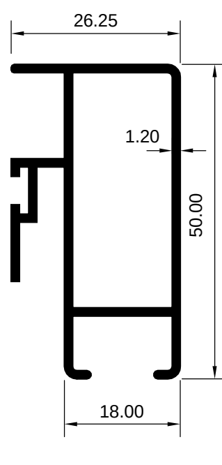
ART 1007973 (KG/MTR = 0.568)
