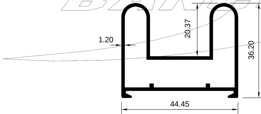
ART 2007916 (KG/MTR = 0.993)
