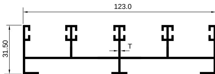
4 TRACK TOP
