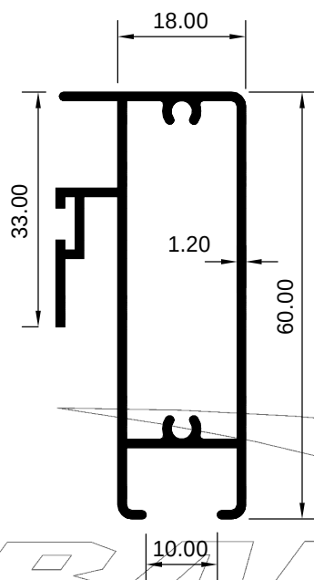
ART 1007843 (KG/MTR = 0.680)
