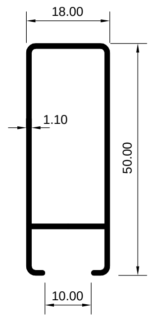
ART 1029005 (KG/MTR = 0.400)
