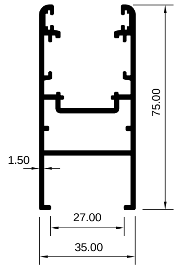
ART 2008072 (KG/MTR = 1.122)
