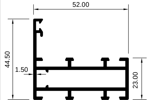
ART 1008071 (KG/MTR = 0.883)
