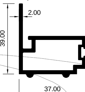
ART 2007810 (KG/MTR = 0.775)
