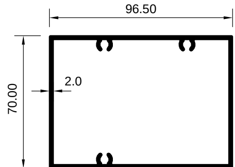
ART 3029013 (KG/MTR = 1.939)
