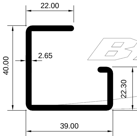
ART 1007941 (KG/MTR = 0.831)
