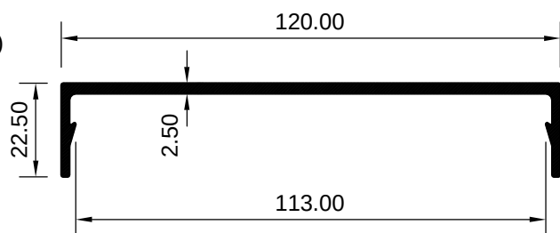
ART 1029168 (KG/MTR = 1.049)
