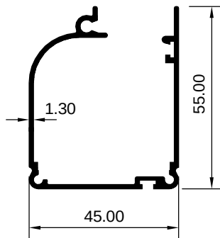
ART 2029099 (KG/MTR = 0.314)
