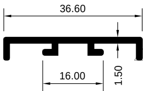
ART 1029045 (KG/MTR = 0.229)
