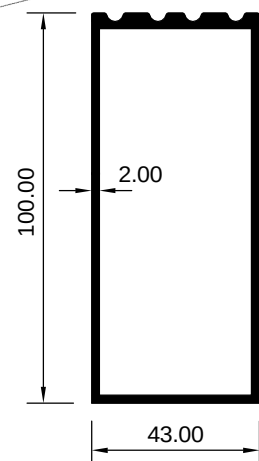
ART 1007808 (KG/MTR = 0.351)
