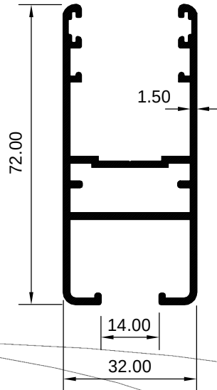
ART 1029181 (KG/MTR = 0.978)
