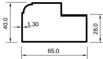
ART 2007994 (KG/MTR = 1.628)
