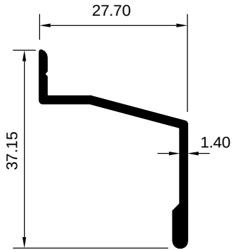
ART 2008028 (KG/MTR = 0.247)
