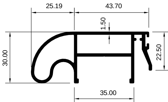
ART 1029405 (KG/MTR = 0.977)
