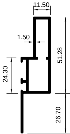
ART 1007986 (KG/MTR = 0.698)
