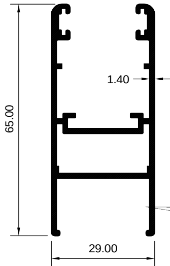
ART 2029339 (KG/MTR = 0.851)
