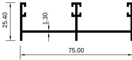
ART 1007829 (KG/MTR = 0.651)
