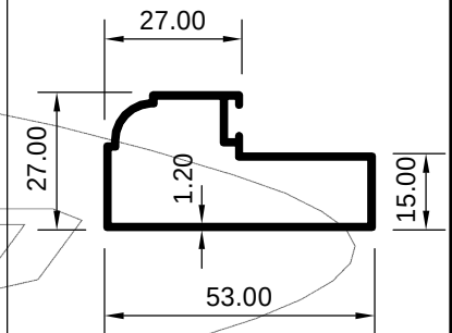
ART 1008049 (KG/MTR = 0.509)
