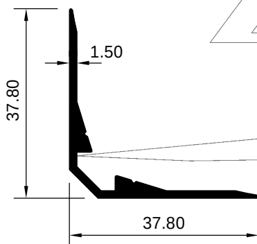
ART 1007848 (KG/MTR = 0.360)
