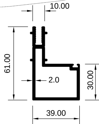
ART 2029352 (KG/MTR = 0.974)
