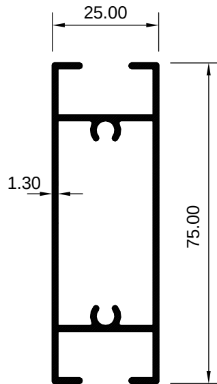
ART 1029421 (KG/MTR = 0.832)
