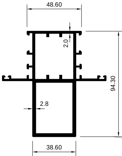
⊗ ART 2029108 (KG/MTR = 2.471)
