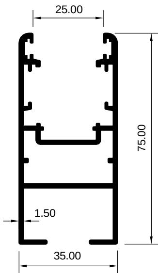
ART 2007995 (KG/MTR = 1.171)
