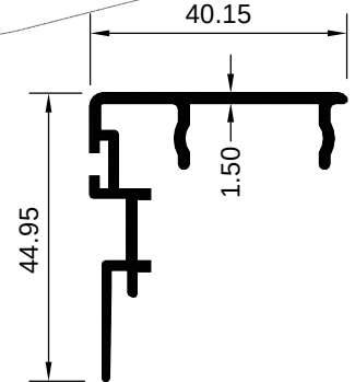
ART 1029182 (KG/MTR = 0.487)
