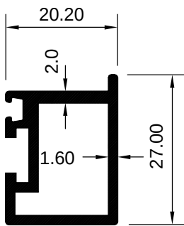
ART 1029104 (KG/MTR = 0.441)
