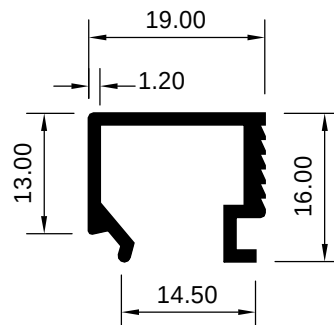
ART 1029234 (KG/MTR = 0.204)
