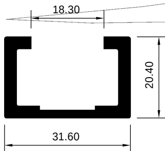
HAD 1007447 (KG/MTR = 0.559)
