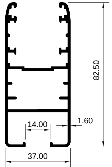
ART 2007967 (KG/MTR = 1.340)
