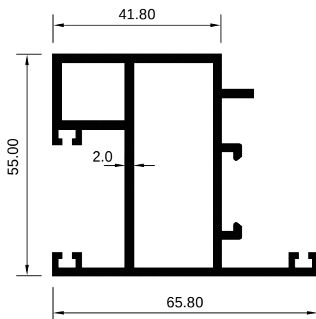
ART 2029337 (KG/MTR = 1.451)
