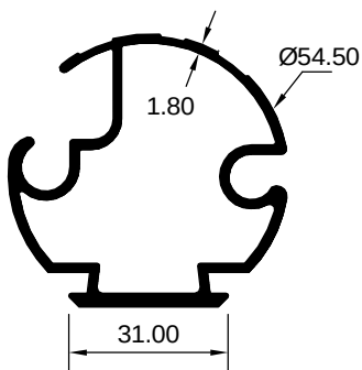
ART 1008004 (KG/MTR = 0.228)
