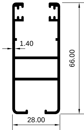
ART 2007887 (KG/MTR = 0.867)
