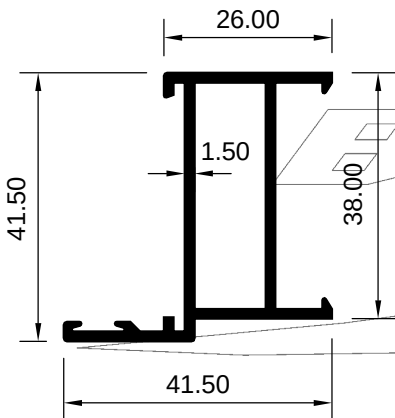
ART 1029034 (KG/MTR = 0.757)
