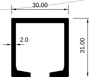
HAD 2007488 (KG/MTR = 0.621)
