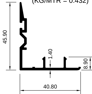
ART 1029267 (KG/MTR = 0.432)
