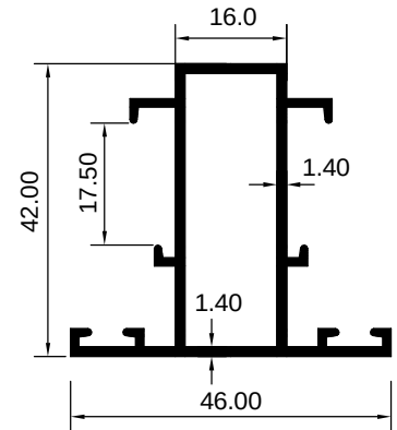
ART 1005578 (KG/MTR = 0.673)
