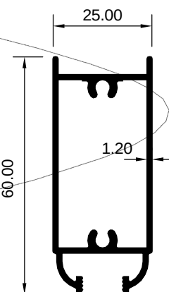
ART 2029220 (KG/MTR = 0.767)
