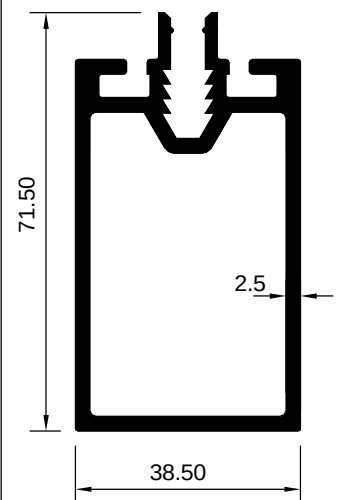
ART 2005461 (KG/MTR = 1.734)
