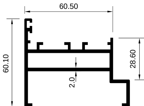
ART 2008043 (KG/MTR = 1.393)
