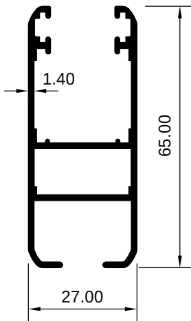
ART 1007870 (KG/MTR = 0.838)
