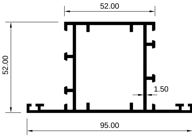
ART 2029215 (KG/MTR = 1.297)
