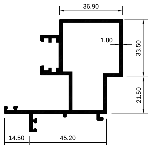
ART 2029343 (KG/MTR = 1.367)
