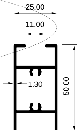
ART 2008086 (KG/MTR = 0.613)
