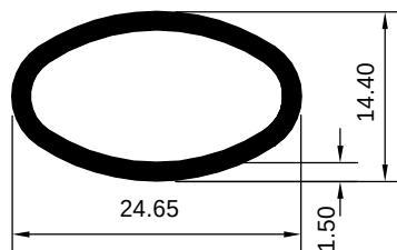
HAD 1007548 (KG/MTR = 0.233)
