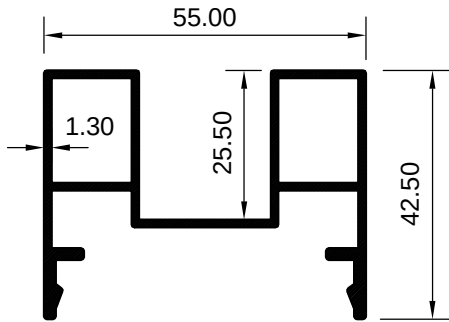
ART 1029115 (KG/MTR = 0.469)
