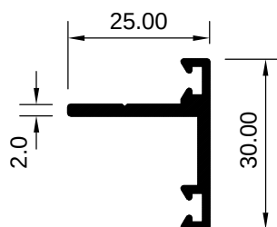
ART 2029099 (KG/MTR = 0.314)
