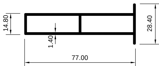
ART 1029317 (KG/MTR = 0.768)
