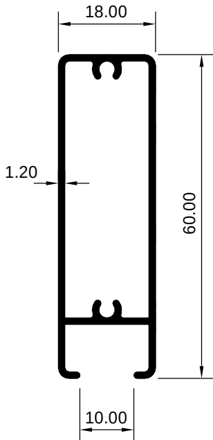
ART 1007842 (KG/MTR = 0.546)
