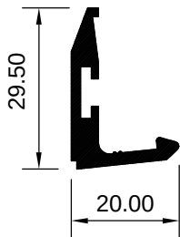
ART 2007939 (KG/MTR = 0.376)
