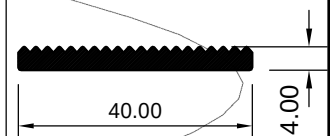
ART 2029351 (KG/MTR = 0.384)
