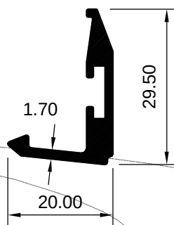
ART 2029072 (KG/MTR = 0.347)
