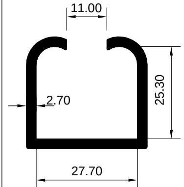
ART 2007950 (KG/MTR = 0.708)
