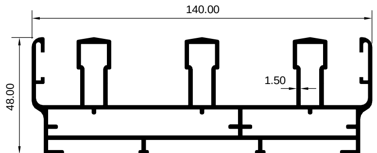
ART 3007998 (KG/MTR = 2.665)
