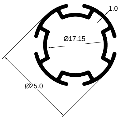
ART 1007722 (KG/MTR = 0.294)
