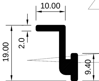
ART 1029143 (KG/MTR = 0.215)
