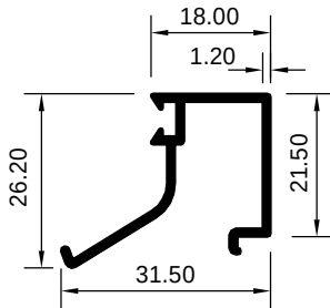
ART 1008067 (KG/MTR = 0.275)
