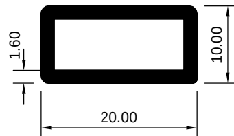
HAD 1007549 (KG/MTR = 0.220)
