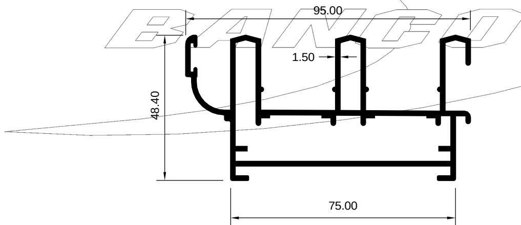
ART 2008026 (KG/MTR = 1.715)
