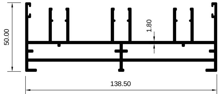
ART 3029340 (KG/MTR = 2.817)
