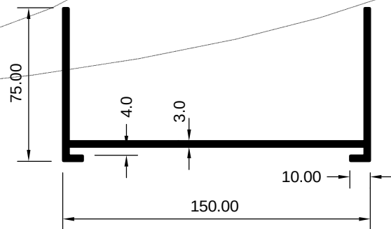
ART 3029171 (KG/MTR = 2.493)
