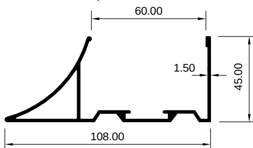
ART 2007782 (KG/MTR = 1.124)
