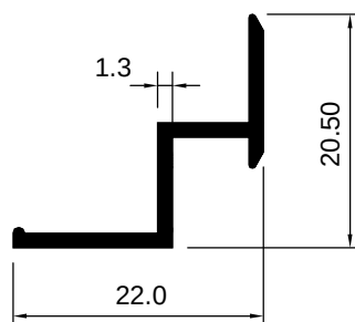
ART 2007719 (KG/MTR = 0.151)
