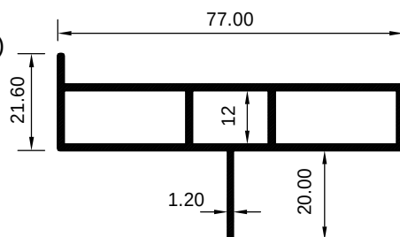
ART 1029321 (KG/MTR = 0.852)
