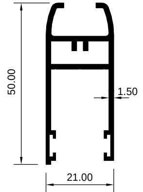
ART 2007832 (KG/MTR = 0.600)
