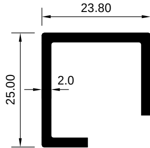
ART 1007769 (KG/MTR = 0.382)
