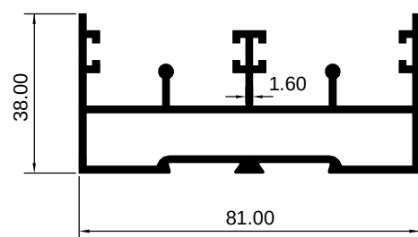
2 TRACK HOLLOW BOTTOM
