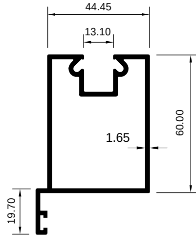
ART 2029030 (KG/MTR = 1.230)
