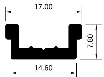
ART 1007896 (KG/MTR = 0.170)
