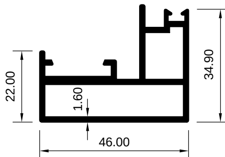
ART 1029223 (KG/MTR = 0.881)
