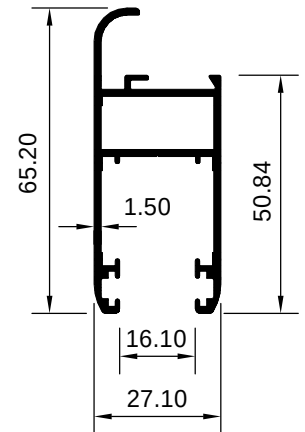
ART 1007791 (KG/MTR = 0.676)
