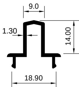
ART 1029224 (KG/MTR = 0.200)
