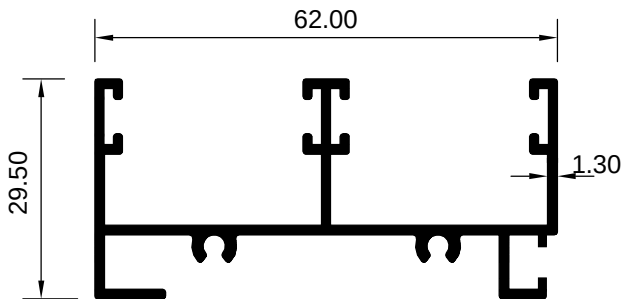
ART 1007897 (KG/MTR = 0.698)
