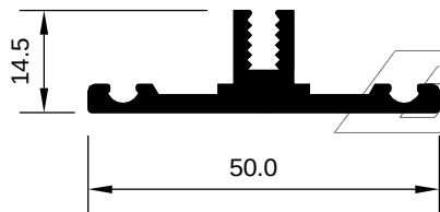
ART 2007795 (KG/MTR = 1.178)
