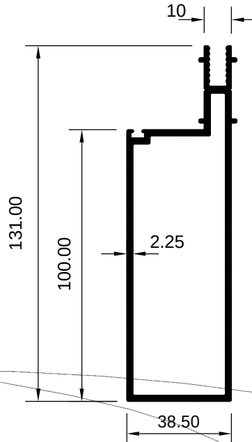
ART 2007946 (KG/MTR = 2.018)
