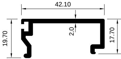
ART 2008046 (KG/MTR = 0.468)
