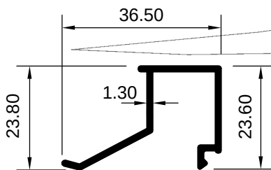
ART 1008024 (KG/MTR = 0.286)
