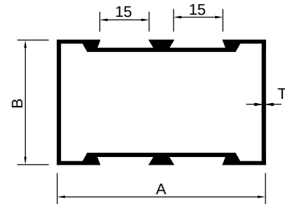
DOUBLE PARTITION
