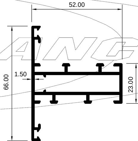
ART 1008069 (KG/MTR = 0.999)
