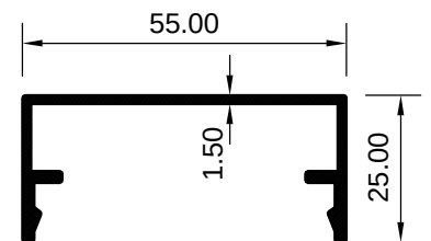
ART 2029113 (KG/MTR = 0.511)
