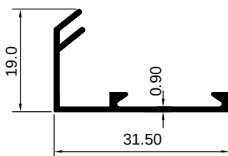
ART 1005709 (KG/MTR = 0.175)
