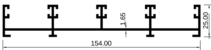
ART 2007766 (KG/MTR = 1.595)
