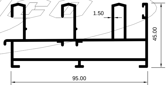
ART 2008073 (KG/MTR = 1.727)
