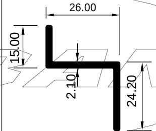
ART 2008008 (KG/MTR = 0.345)
