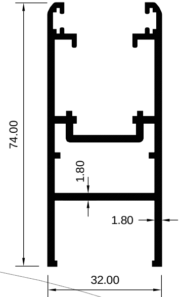
ART 1029182 (KG/MTR = 0.487)
