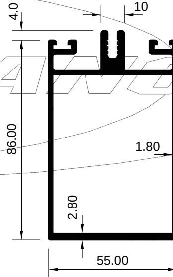
ART 1029106 (KG/MTR = 0.737)
