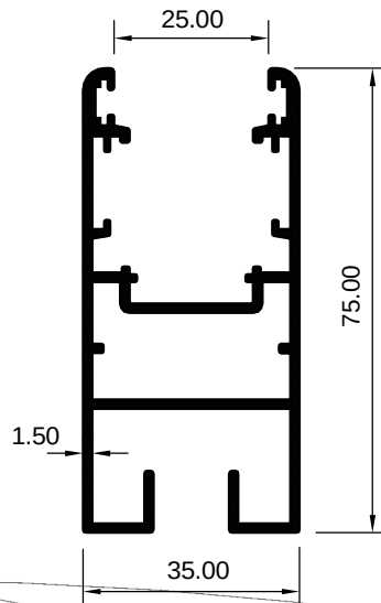
ART 2029262 (KG/MTR = 1.251)
