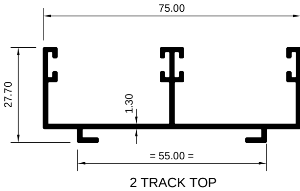
ART 1029040 (KG/MTR = 0.668)
