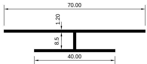
ART 1029316 (KG/MTR = 0.118)
