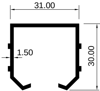
ART 1007941 (KG/MTR = 0.831)
