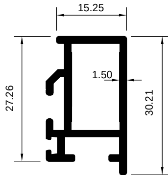
ART 1029288 (KG/MTR = 0.396)
