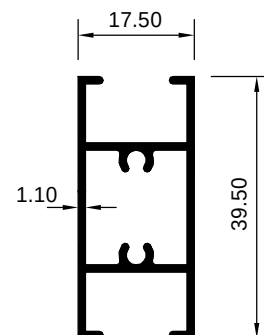
ART 2007828 (KG/MTR = 0.408)
