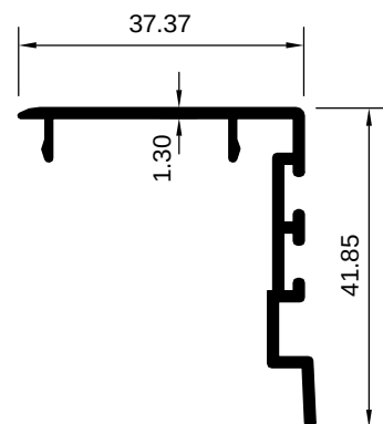
ART 1008082 (KG/MTR = 0.368)
