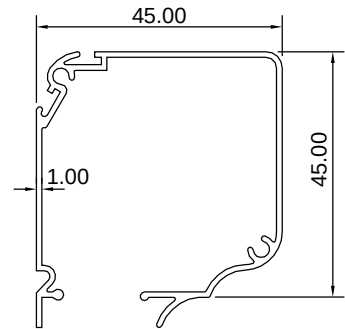
ART 1007724 (KG/MTR = 0.520)
