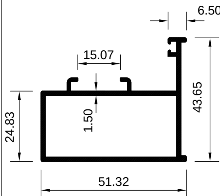
ART 1029106 (KG/MTR = 0.737)
