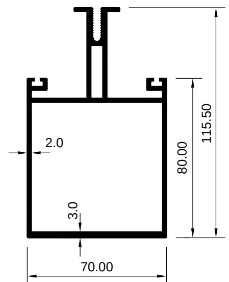
ART 2029140 (KG/MTR = 2.574)
