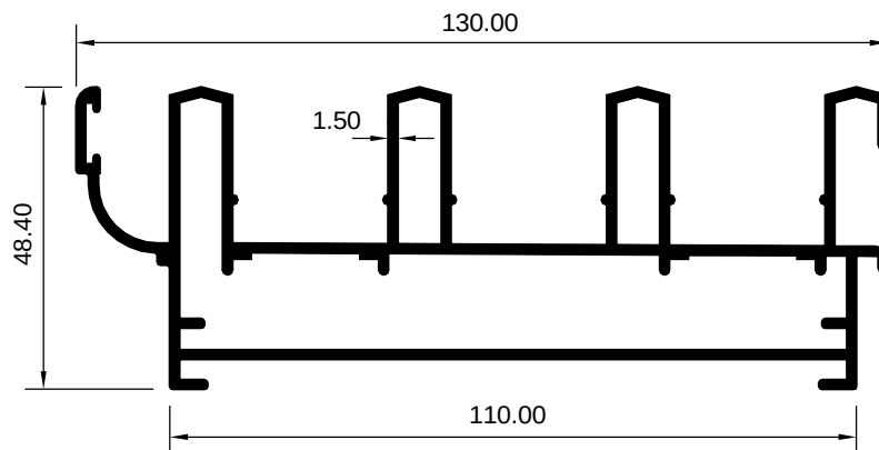
ART 3008027 (KG/MTR = 2.222)
