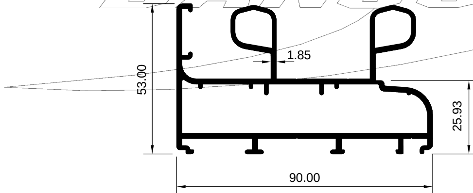
ART 3007968 (KG/MTR = 2.900)
