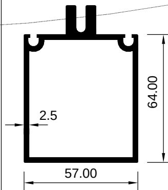
ART 2007865 (KG/MTR = 2.041)
