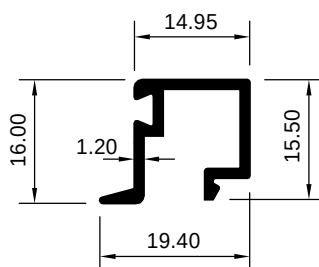
ART 1029228 (KG/MTR = 0.189)
