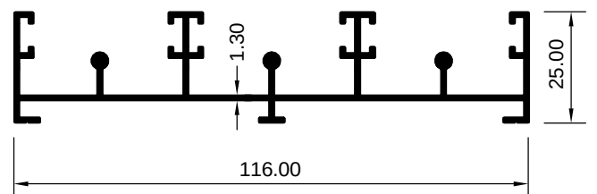
ART 2007797 (KG/MTR = 1.267)
