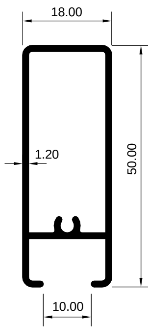
ART 1007972 (KG/MTR = 0.458)
