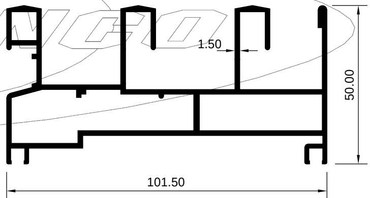
ART 2029411 (KG/MTR = 1.606)
