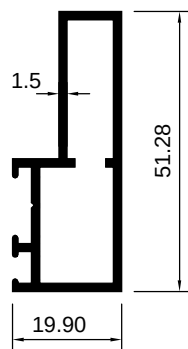
ART 1007710 (KG/MTR = 0.591)
