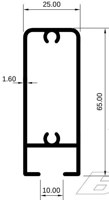
ART 1007844 (KG/MTR = 0.868)
