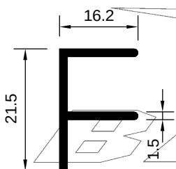
ART 2003223 (KG/MTR = 0.214)
