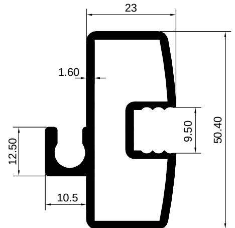
ART 2005580 (KG/MTR = 0.885)
