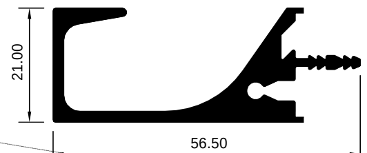
HAD 2007414 (KG/MTR = 0.835)
