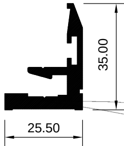
ART 2007822 (KG/MTR = 0.693)
