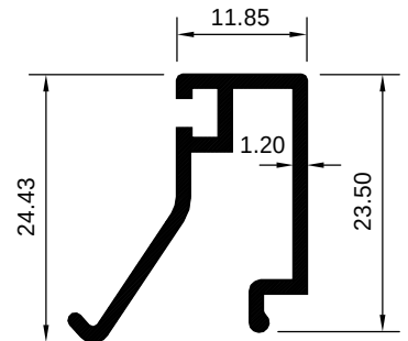
ART 2029336 (KG/MTR = 1.337)
