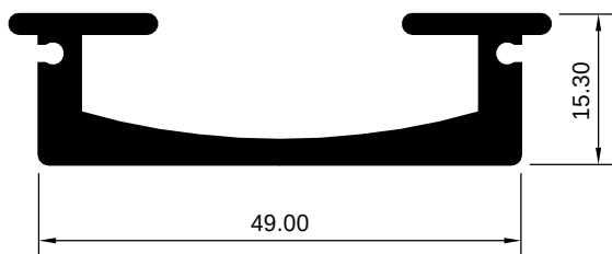
HAD 1007545 (KG/MTR = 0.544)
