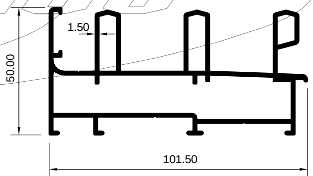
ART 2007985 (KG/MTR = 1.920)
