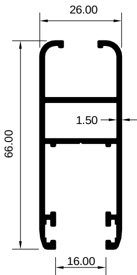
ART 1007982 (KG/MTR = 0.852)
