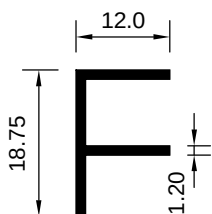
ART 1002933 (KG/MTR = 0.126)
