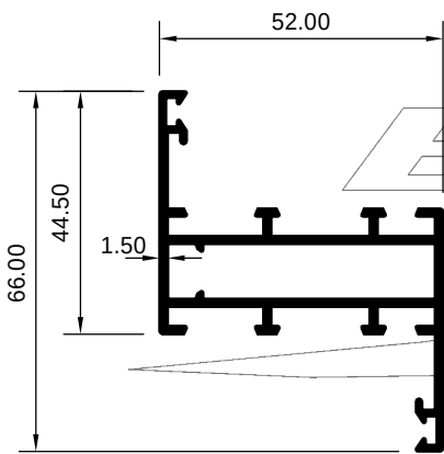
ART 1008070 (KG/MTR = 0.999)
