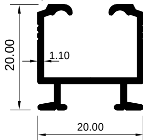
ART 1008004 (KG/MTR = 0.228)
