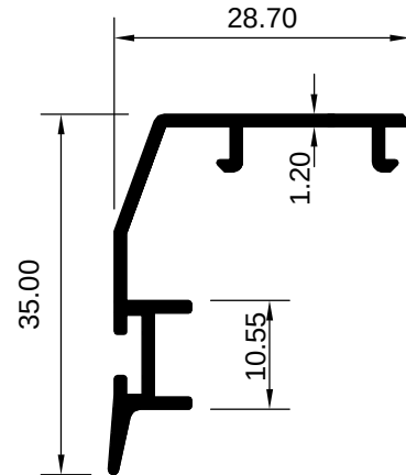
ART 1007914 (KG/MTR = 0.284)
