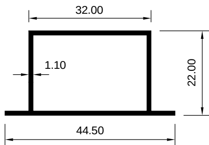
ART 1007768 (KG/MTR = 0.344)
