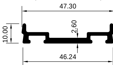
ART 1008075 (KG/MTR = 0.390)
