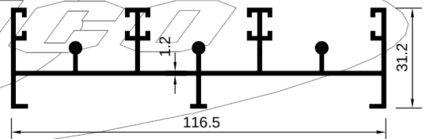
ART 2007702 (KG/MTR = 1.110)
