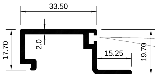
ART 1029355 (KG/MTR = 0.484)
