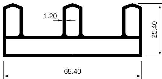
ART 1029365 (KG/MTR = 0.825)
