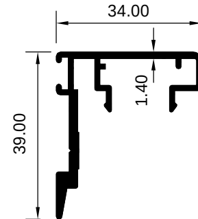
ART 1007888 (KG/MTR = 0.490)
