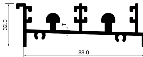
2 TRACK BOTTOM
