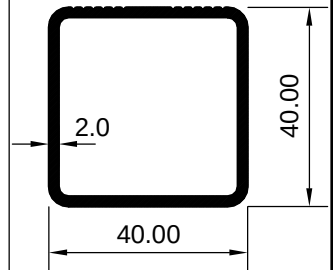
ART 2029165 (KG/MTR = 0.785)
