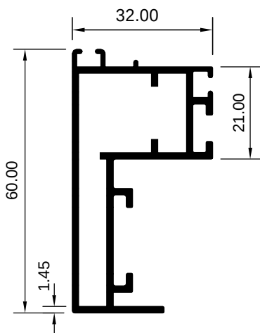
ART 1007894 (KG/MTR = 0.870)
