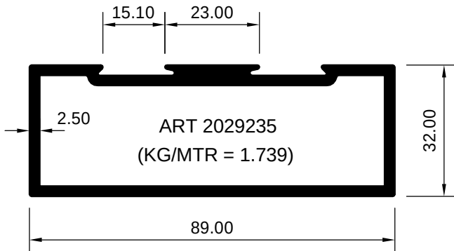
SINGLE PARTITION
