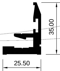
ART 2007940 (KG/MTR = 0.693)
