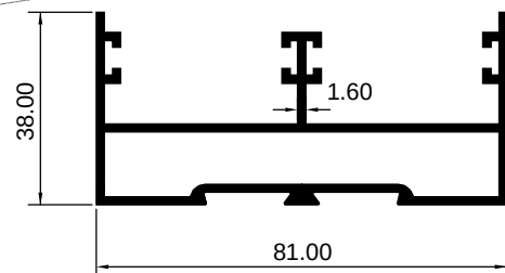
2 TRACK HOLLOW TOP
