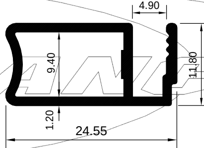
ART 1029270 (KG/MTR = 0.239)
