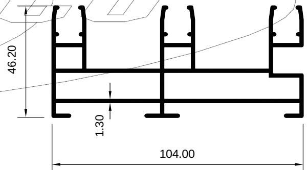
ART 2029420 (KG/MTR = 1.687)
