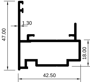
ART 2008094 (KG/MTR = 0.634)
