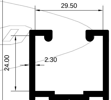
ART 2007950 (KG/MTR = 0.708)
