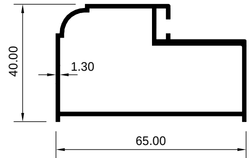
ART 1008049 (KG/MTR = 0.509)
