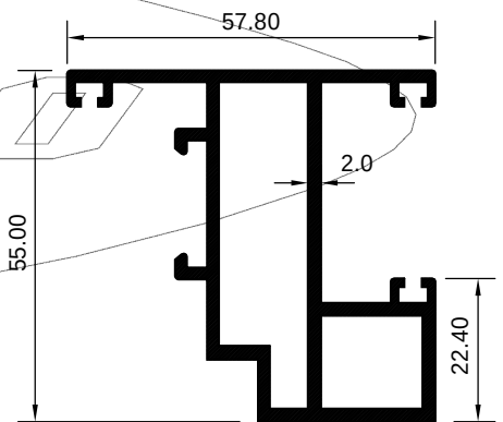
ART 2029336 (KG/MTR = 1.337)
