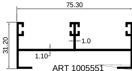
ART 1005551 (KG/MTR = 0.687)
