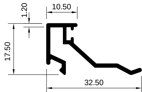
ART 1008000 (KG/MTR = 0.222)
