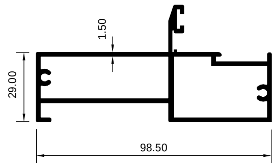
ART 2008091 (KG/MTR = 1.409)
