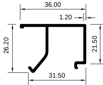
ART 1008068 (KG/MTR = 0.306)
