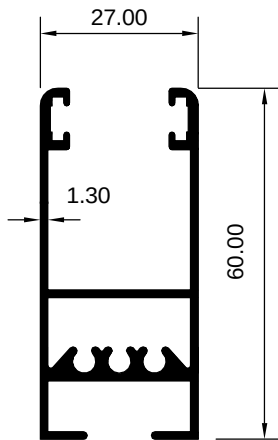
ART 1007788 (KG/MTR = 0.852)
