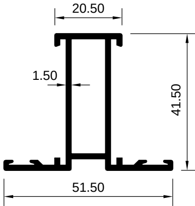
ART 1029229 (KG/MTR = 0.672)
