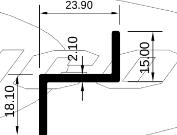
ART 2008007 (KG/MTR = 0.298)
