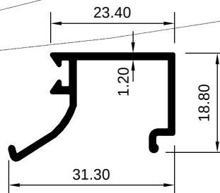
ART 1008058 (KG/MTR = 0.235)
