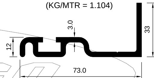
ART 2005575 (KG/MTR = 1.104)
