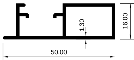
ART 2007810 (KG/MTR = 0.775)
