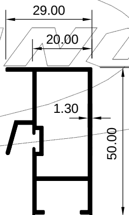
ART 1007909 (KG/MTR = 0.600)
