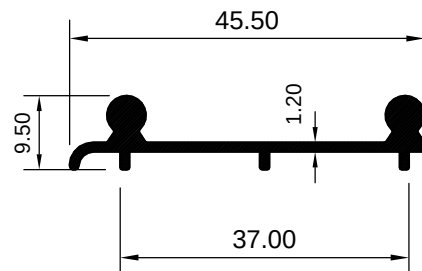
ART 2029048 (KG/MTR = 0.306)
