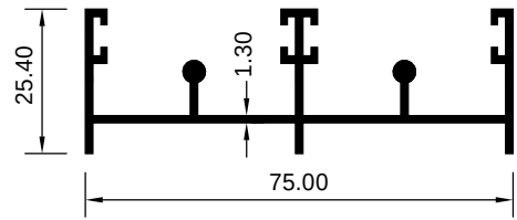
ART 1007830 (KG/MTR = 0.759)
