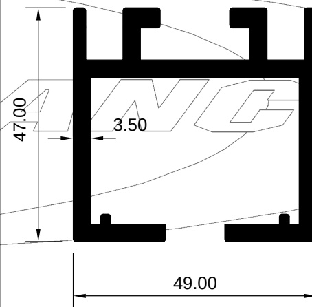
ART 2007942 (KG/MTR = 1.815)
