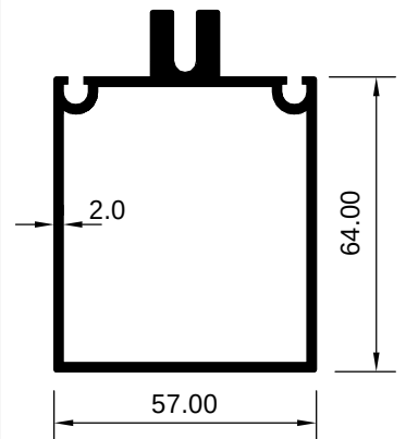
ART 2007857 (KG/MTR = 1.742)
