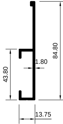
ART 2029332 (KG/MTR = 0.611)
