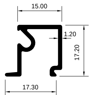
ART 1029227 (KG/MTR = 0.381)
