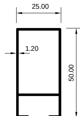
ART 1007952 (KG/MTR = 0.506)
