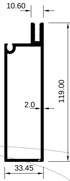
ART 2029260 (KG/MTR = 1.742)
