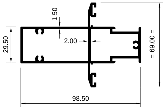
ART 1008092 (KG/MTR = 1.036)
