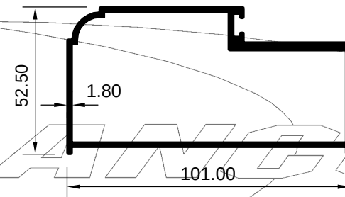
ART 2005574 (KG/MTR = 1.191)
