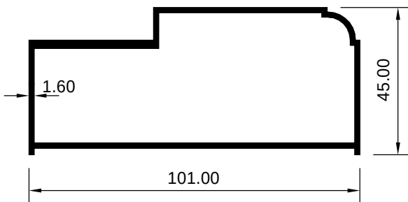
ART 2007860 (KG/MTR = 1.311)
