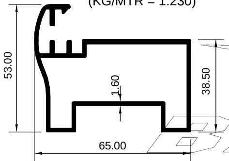
ART 2007783 (KG/MTR = 1.230)
