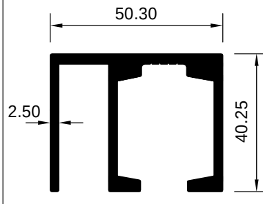
ART 2007855 (KG/MTR = 1.501)
