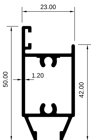
ART 1008089 (KG/MTR = 0.564)
