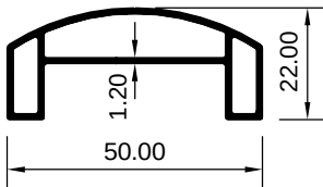
ART 1007847 (KG/MTR = 0.324)
