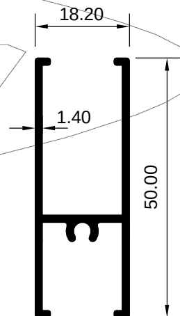
ART 1007911 (KG/MTR = 0.488)
