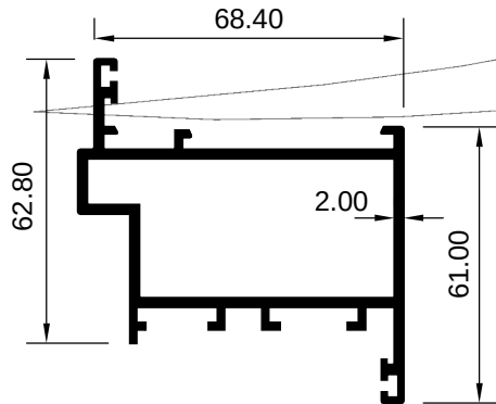
ART 2008045 (KG/MTR = 1.579)
