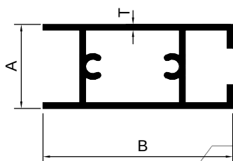
TOP-BOTTOM
