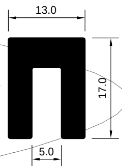
HAD 2007535 (KG/MTR = 0.434)
