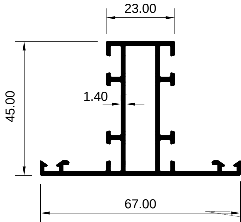
ART 1007891 (KG/MTR = 0.902)
