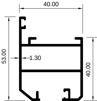
ART 1029034 (KG/MTR = 0.757)
