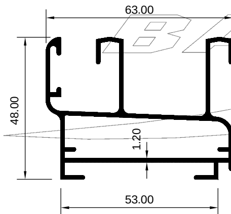
ART 2007790 (KG/MTR = 0.983)
