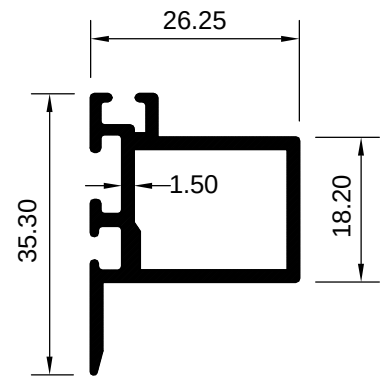
ART 1029328 (KG/MTR = 0.470)
