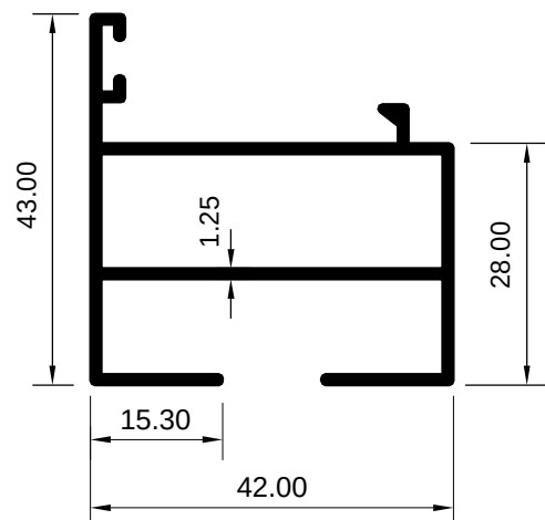
ART 2008053 (KG/MTR = 0.655)
