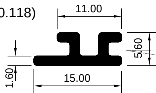
ART 2029291 (KG/MTR = 2.158)
