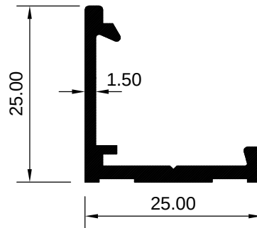
ART 1029144 (KG/MTR = 0.439)
