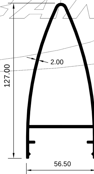
ART 2029159 (KG/MTR = 1.763)
