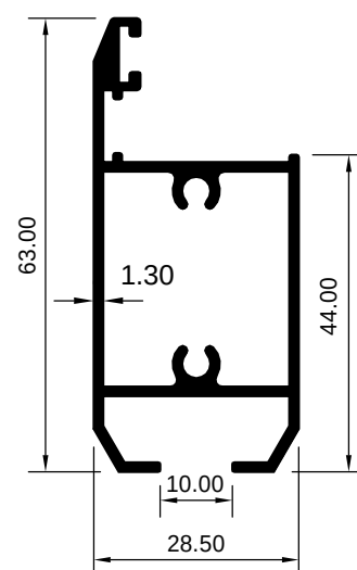
ART 2029220 (KG/MTR = 0.767)
