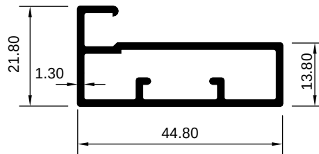
ART 1007980 (KG/MTR = 0.496)
