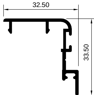
ART 1007789 (KG/MTR = 0.298)
