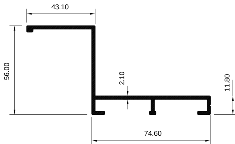
ART 2029329 (KG/MTR = 1.166)
