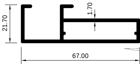
HAD 1034008 (KG/MTR = 0.421)
