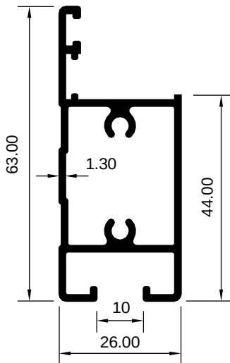
ART 2029221 (KG/MTR = 0.747)
