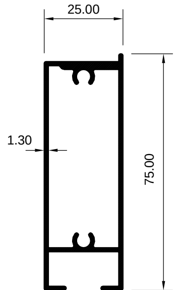
ART 1029422 (KG/MTR = 0.843)
