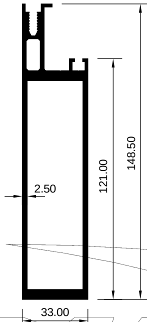
ART 2007865 (KG/MTR = 2.041)
