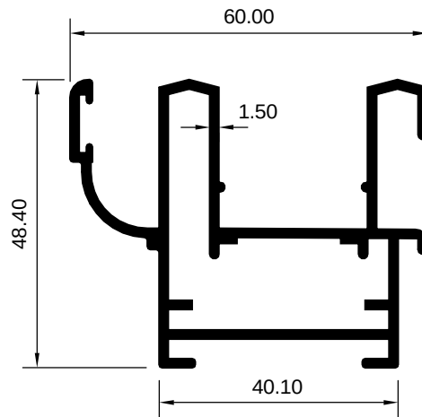
ART 1008025 (KG/MTR = 1.163)
