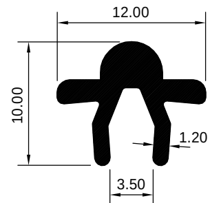
ART 1029316 (KG/MTR = 0.118)
