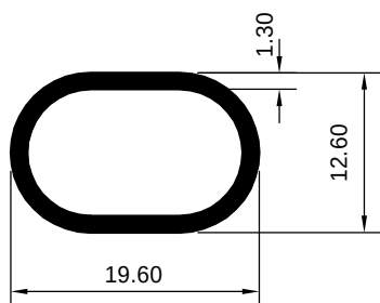
HAD 1007547 (KG/MTR = 0.173)
