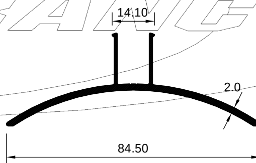
ART 1029279 (KG/MTR = 0.571)
