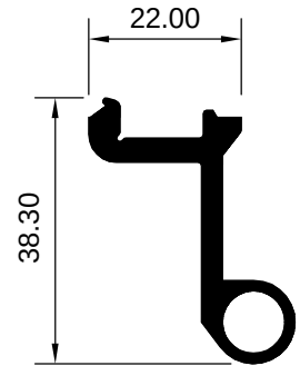
ART 1007959 (KG/MTR = 0.596)
