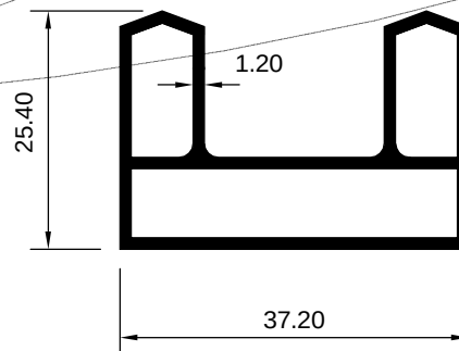
ART 1007812 (KG/MTR = 0.523)
