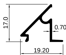
ART 1007720 (KG/MTR = 0.094)
