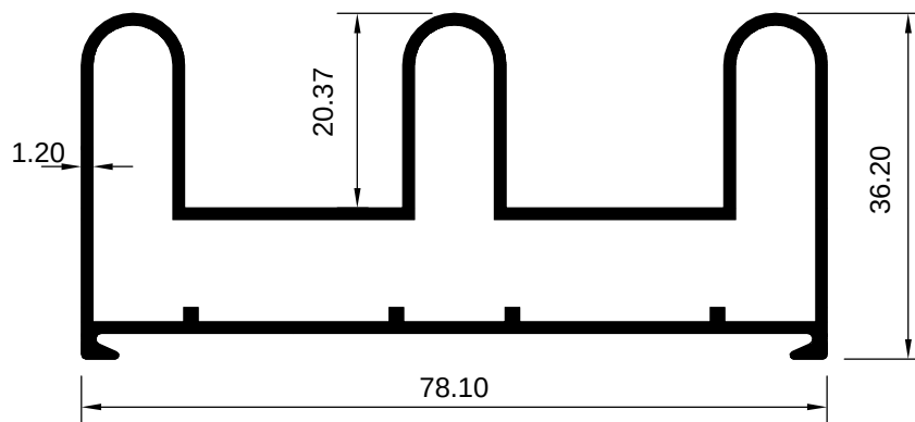
ART 2007916 (KG/MTR = 0.993)
