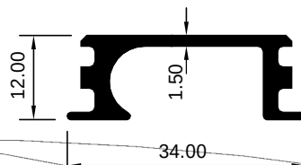
HAD 2007411 (KG/MTR = 0.323)
