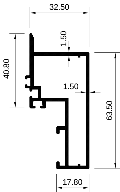
ART 1029346 (KG/MTR = 0.963)
