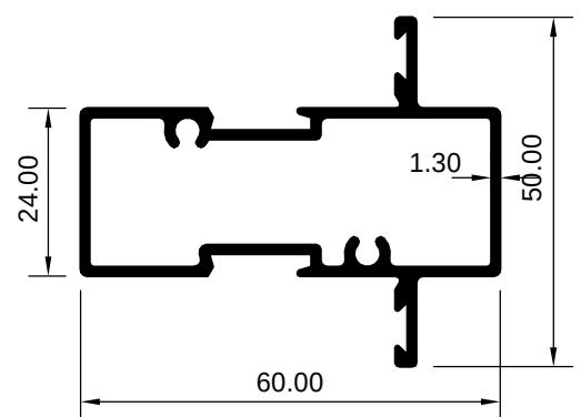
ART 1029233 (KG/MTR = 0.837)
