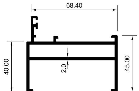
ART 2008042 (KG/MTR = 1.401)
