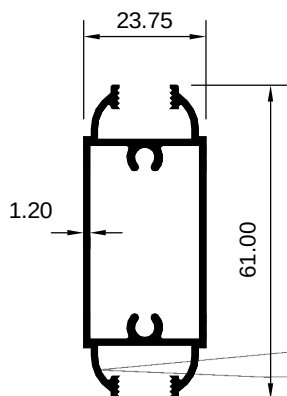
ART 1007787 (KG/MTR = 0.680)
