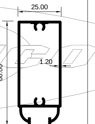
ART 1008050 (KG/MTR = 0.653)
