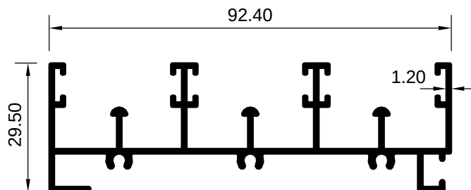
ART 1007988 (KG/MTR = 1.021)
