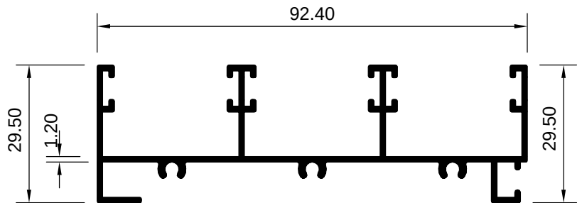
ART 1007899 (KG/MTR = 0.910)
