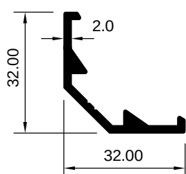
ART 2007813 (KG/MTR = 0.950)
