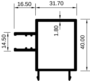
ART 1029342 (KG/MTR = 0.865)
