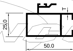
INTER LOCK
