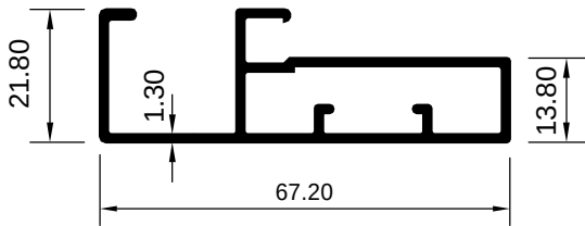
OFS 1009065 (KG/MTR = 0.790)
