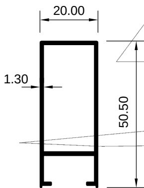
ART 1007908 (KG/MTR = 0.492)
