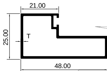
P SECTION
