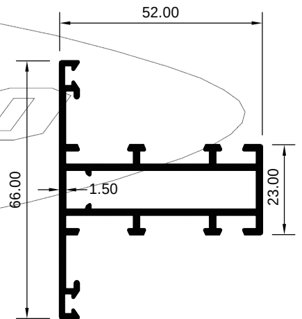
ART 1029357 (KG/MTR = 0.999)
