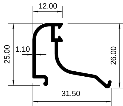
ART 1007970 (KG/MTR = 0.246)
