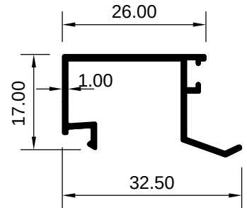
ART 1007936 (KG/MTR = 0.223)
