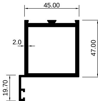
ART 2005574 (KG/MTR = 1.191)
