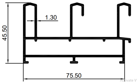
3 TRACK
