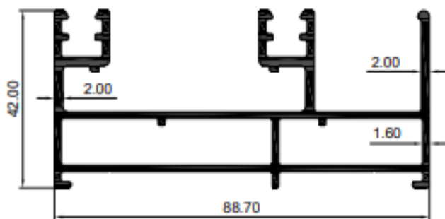
32SS003 16' = 7.800 KG
