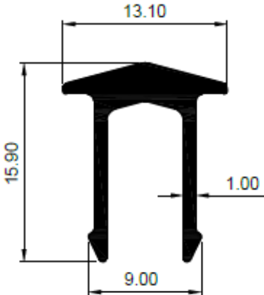
TRACK RAIL V TYPE
