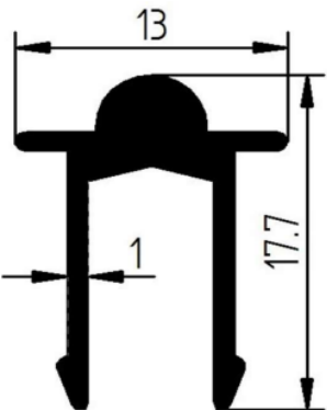
TRACK RAIL U TYPE
