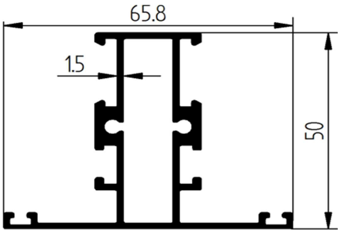
65MM MULLION
