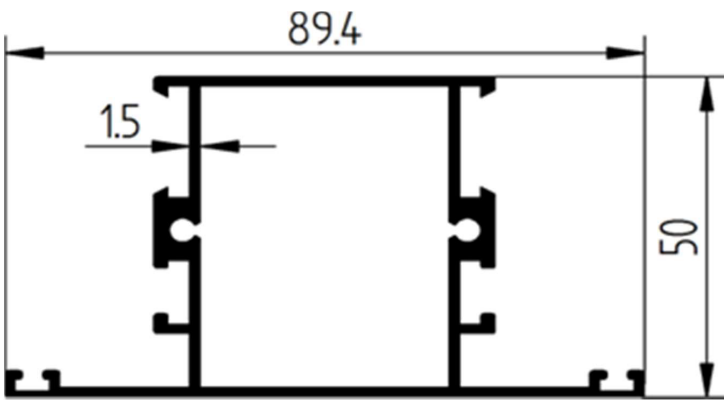
90MM MULLION
