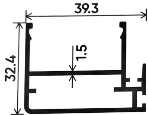
32SS002 16' = 2.900 KG
