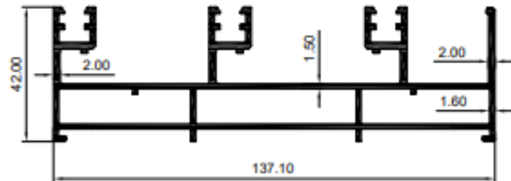
32SS004 16' = 11.300 KG
