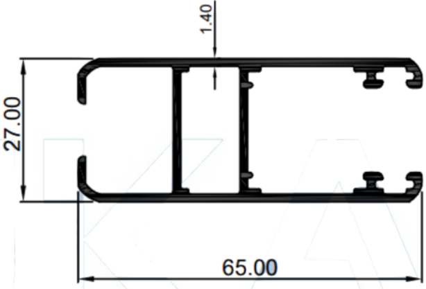
SGU HANDLE
