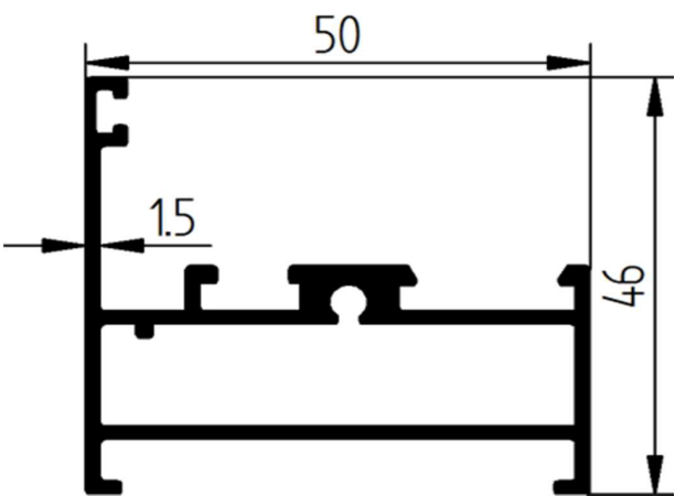
FRAME
