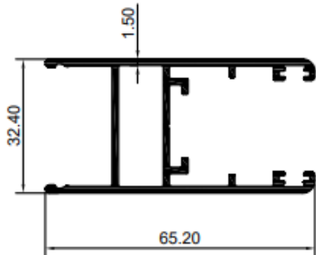
32SS001 16' = 4.900 KG
