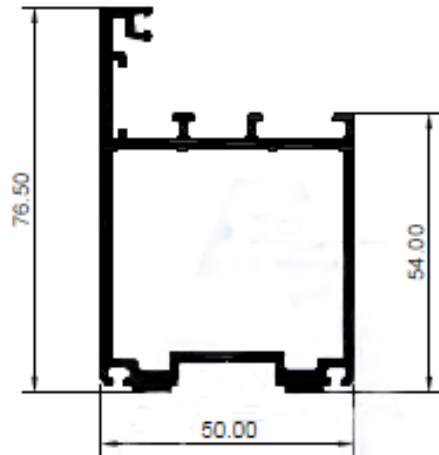
SHUTTER
