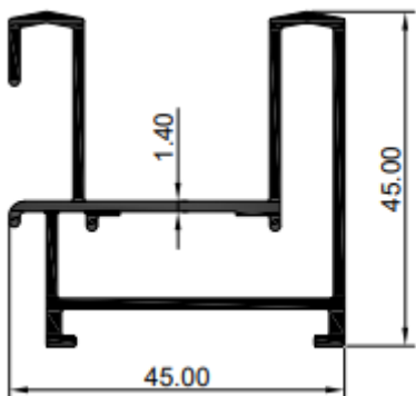
2 TRACK
